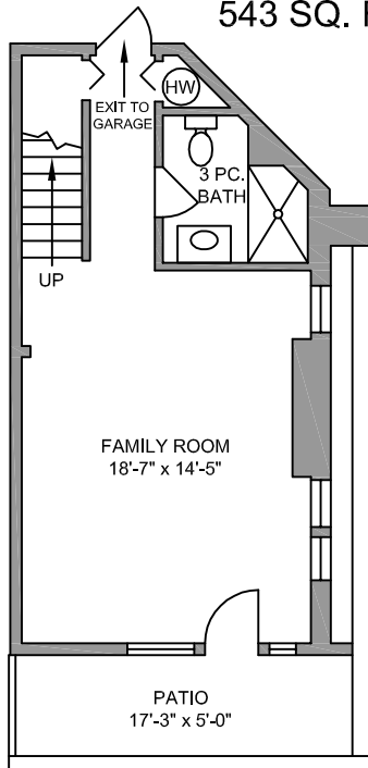
LOWER FLOOR 543 SQ. FT.
